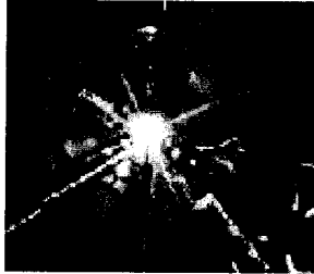
Inertial Confinement
