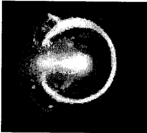
Magnetic Confinement
