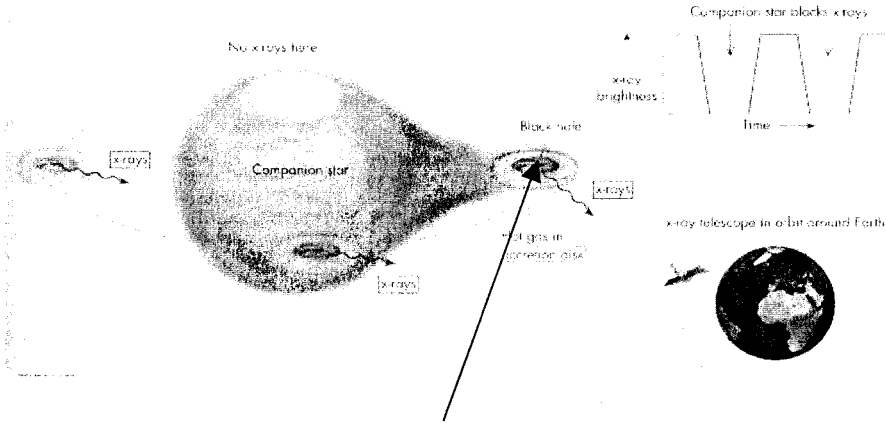
FIGURE 14-14 Black holes may reveal themselves by the x-rays emitted by gas orbiting them in an accretion disk.
