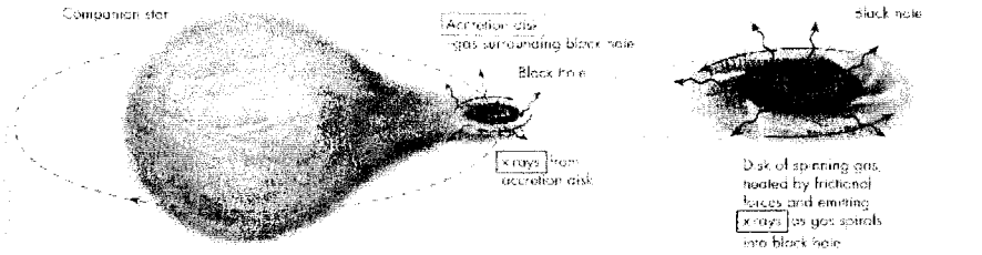
FIGURE 14-14 Black holes may reveal themselves by the x-rays emitted by gas orbiting them in an accretion disk.
