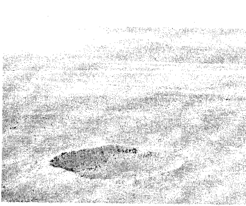
Crater in northern Arizona, made by an asteroid that struck earth (Courtesy of Arizona Tourism)
